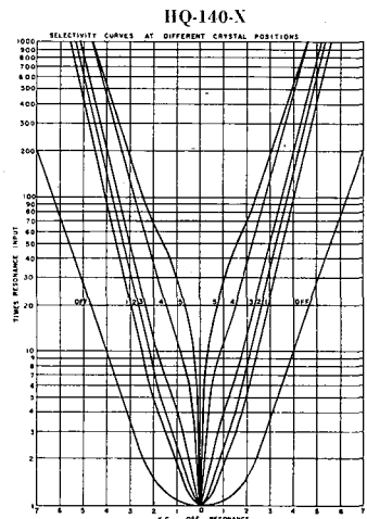
Fig. 10—Selectivity Curves.
